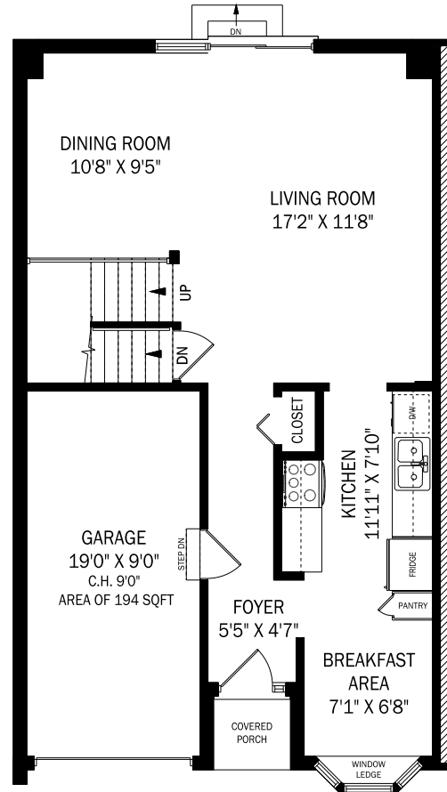
CEILING HEIGHT 8'0" MAIN FLOOR - 639 SQUARE FEET
